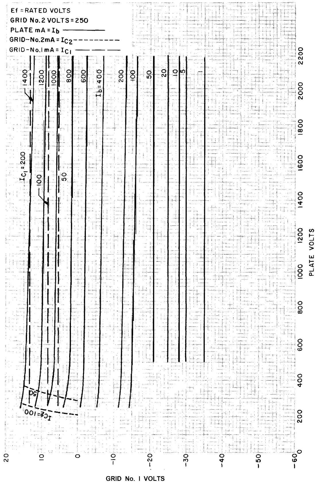
Figure 5 - Typical constant-current characteristics For Grid-No. 2 Voltage = 250 Volts
